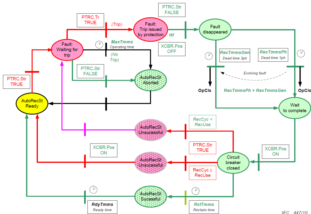
Figure G.1 – Diagram of autorecloser function
